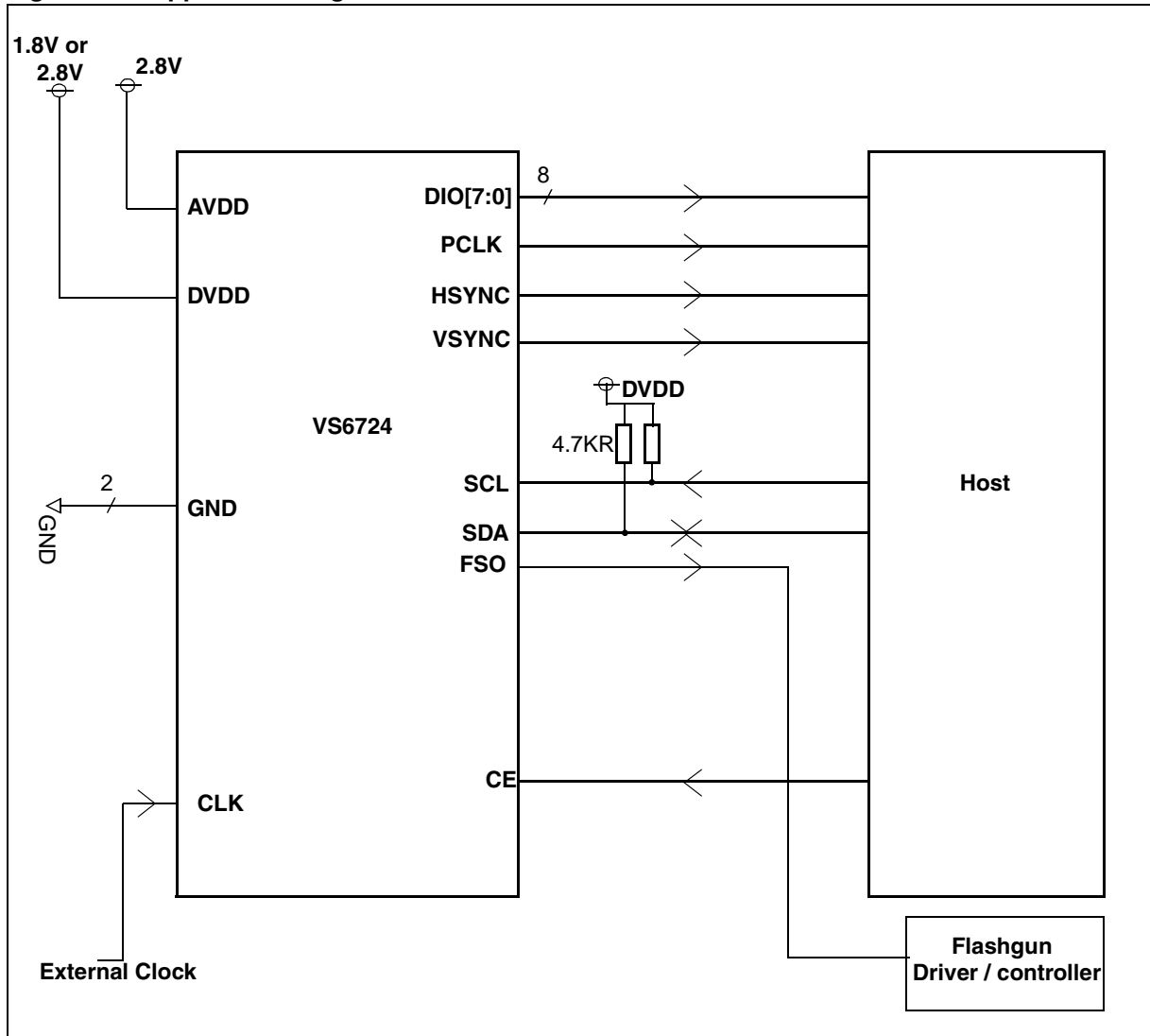
Figure 44. Application diagram
